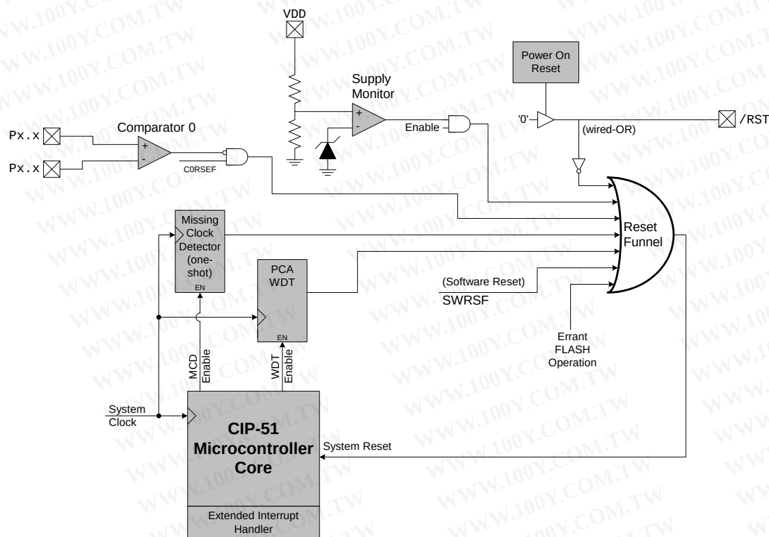
Figure 9.1. Reset Sources
