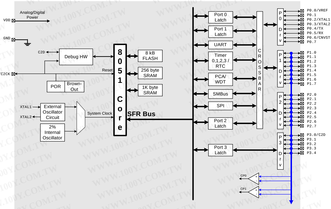
Figure 1.5. C8051F314 Block Diagram
