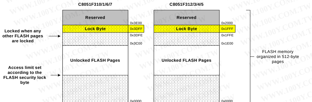
Figure 10.1. Flash Program Memory Map
