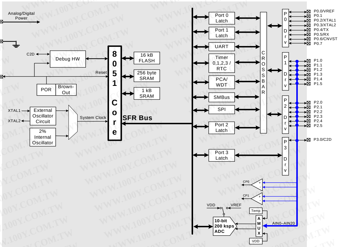
Figure 1.7. C8051F316 Block Diagram
