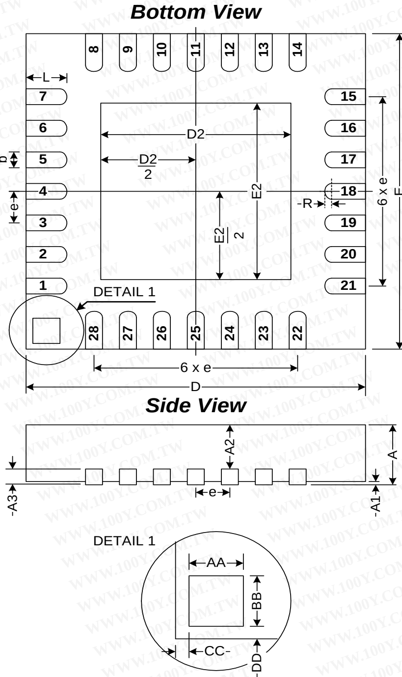
Figure 4.4. QFN-28 Package Drawing
